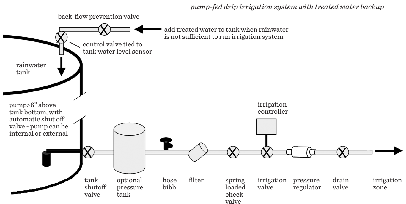
Figure 10e. Pump-fed Drip Irrigation System with Treated Water Backup: The most complex distribution system is drip irrigating plants using pressurized rainwater when it is available, and using treated water as a backup supply when rainwater is low. There are two ways to accomplish this: 1) when rainwater gets low in the tank, add treated water to the top of the tank, then continue to supply the drip irrigation system using water from the tank; or 2) when rainwater gets low in the tank, automatically switch to treated water to directly supply the drip irrigation system. Use this system when the on-going demands of the irrigation system require a back-up water supply to keep the system operating automatically on schedule. Note: When interconnecting treated water and rainwater systems, it is imperative that your system automatically prevents any cross-contamination between rainwater and treated water.
