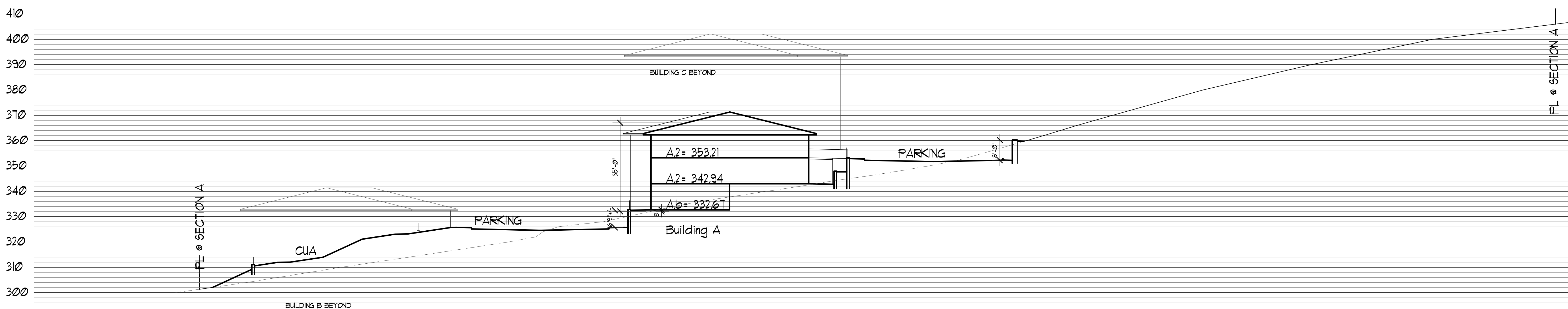
SITE SECTION A: BUILDING A: 1"=20'
