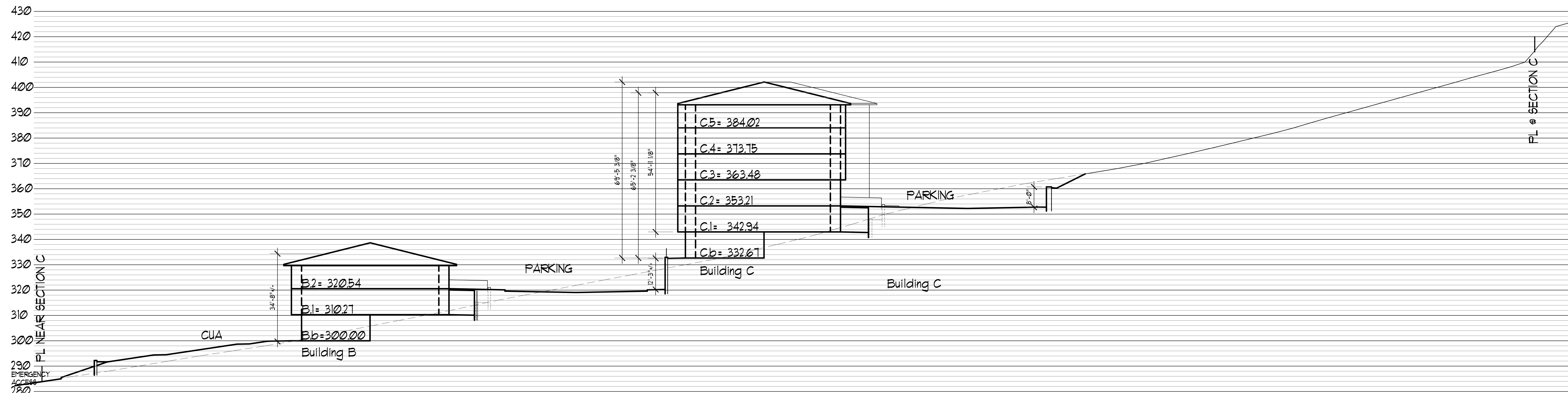
SITE SECTION C: BUILDINGS B & C: 1"=20'
