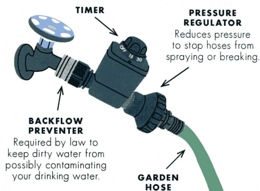
Diagram of connection set-up at the faucet for a soaker hose
