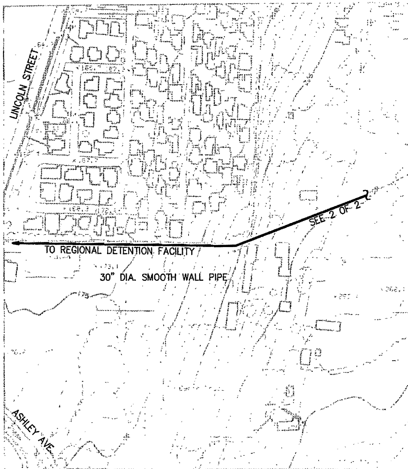
SCHEMATIC LINCOLN CREEK PROBLEM NO. 7
