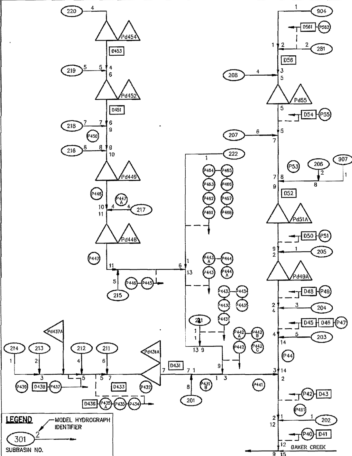
HYDROLOGIC MODEL SCHEMATIC FOR SPRING CREEK BASIN
