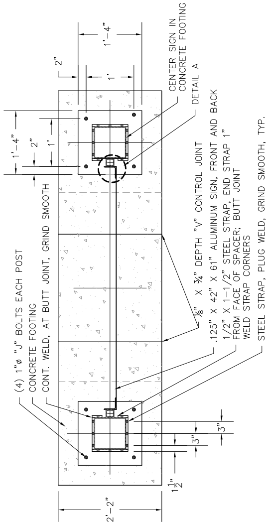
PLAN VIEW (SCALE 1/2" = 1'-0")
