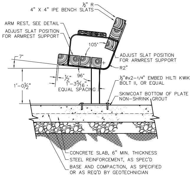
SIDE SECTION
